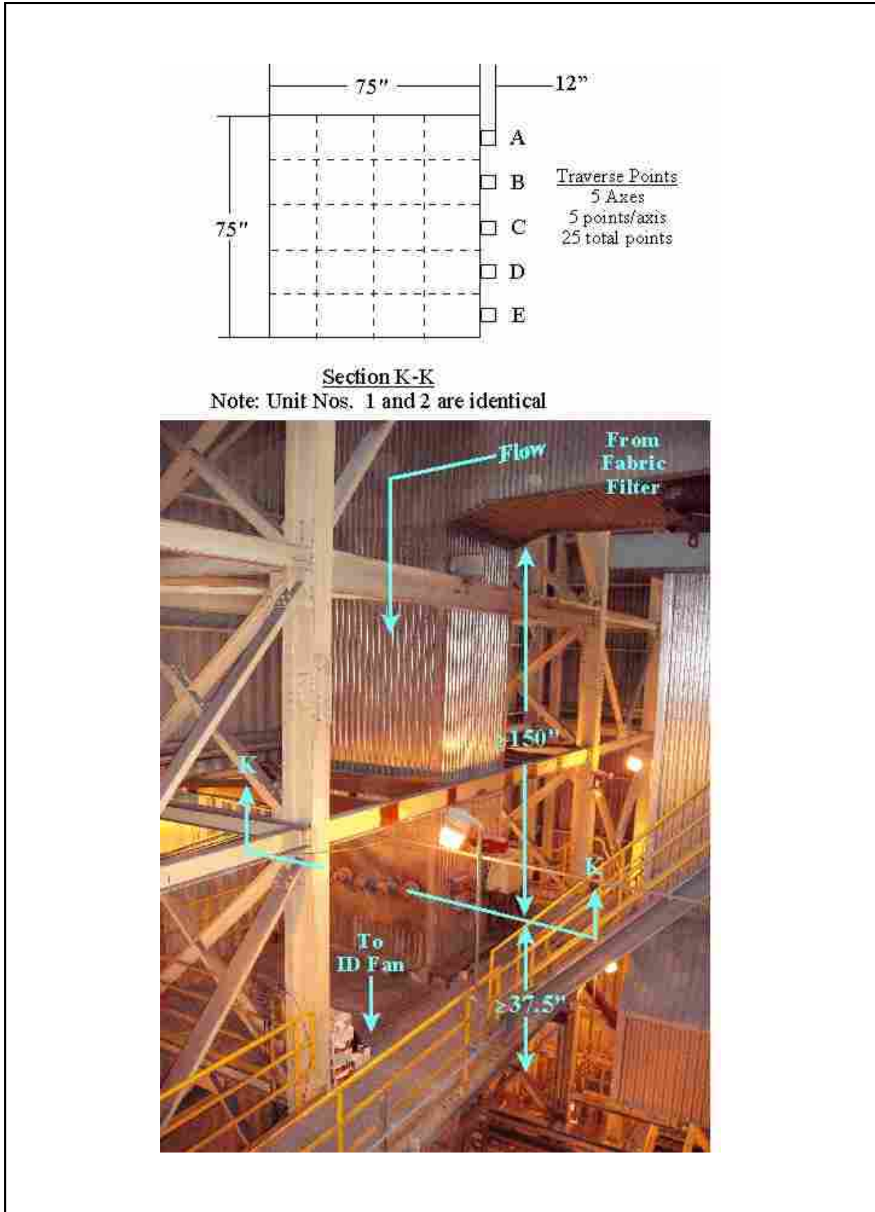
Figure 4.2 Schematic of Unit Nos. 1 and 2 FF outlet sampling location.
