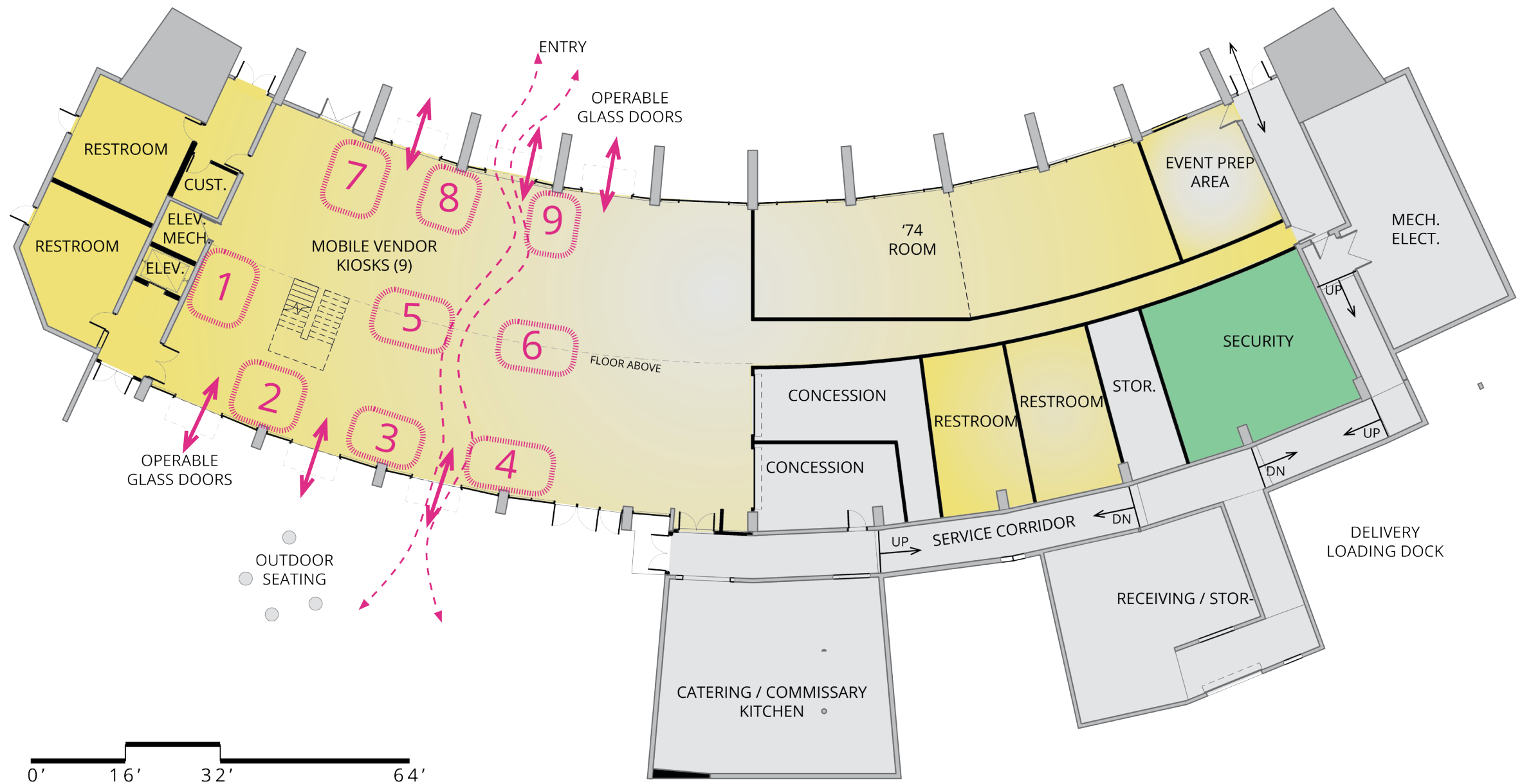
west building conceptual plan Level 1
