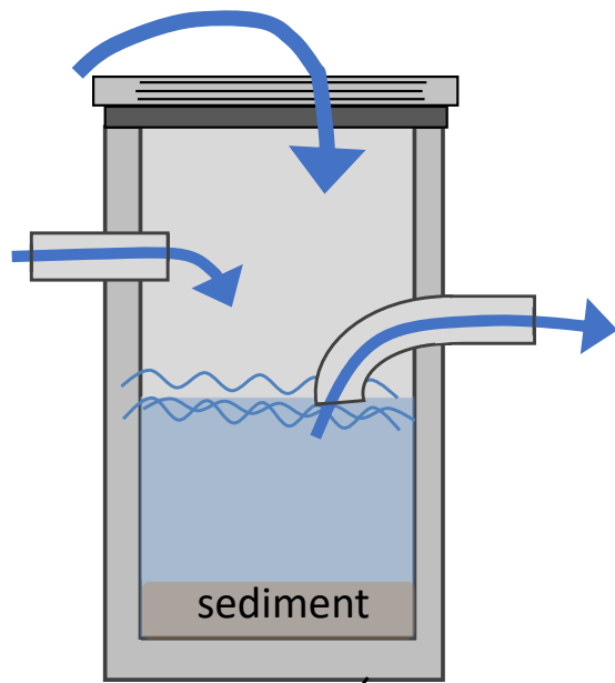
General Catch Basin
