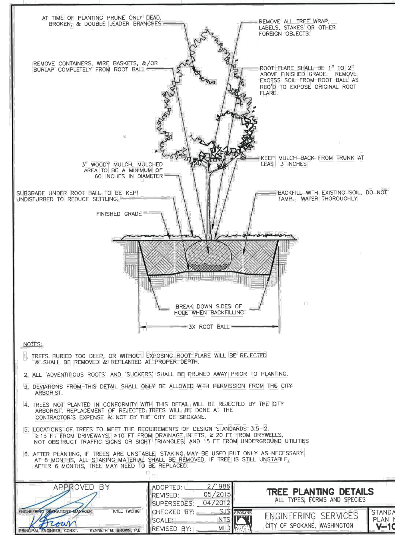
1 TREE PLANTING DETAIL L1.0 NTS
