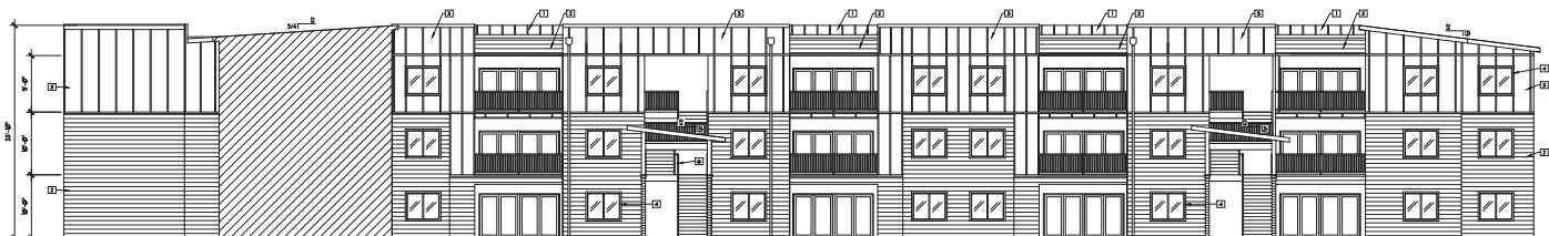
EAST ELEVATION 1/8" = 1'-0"
