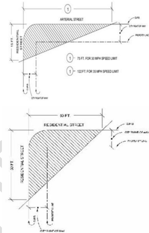
FIGURE 12a Vision Clearance Area
