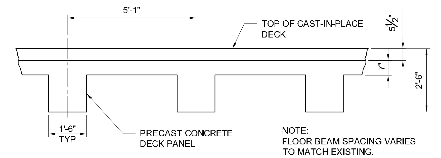
(C) Section
