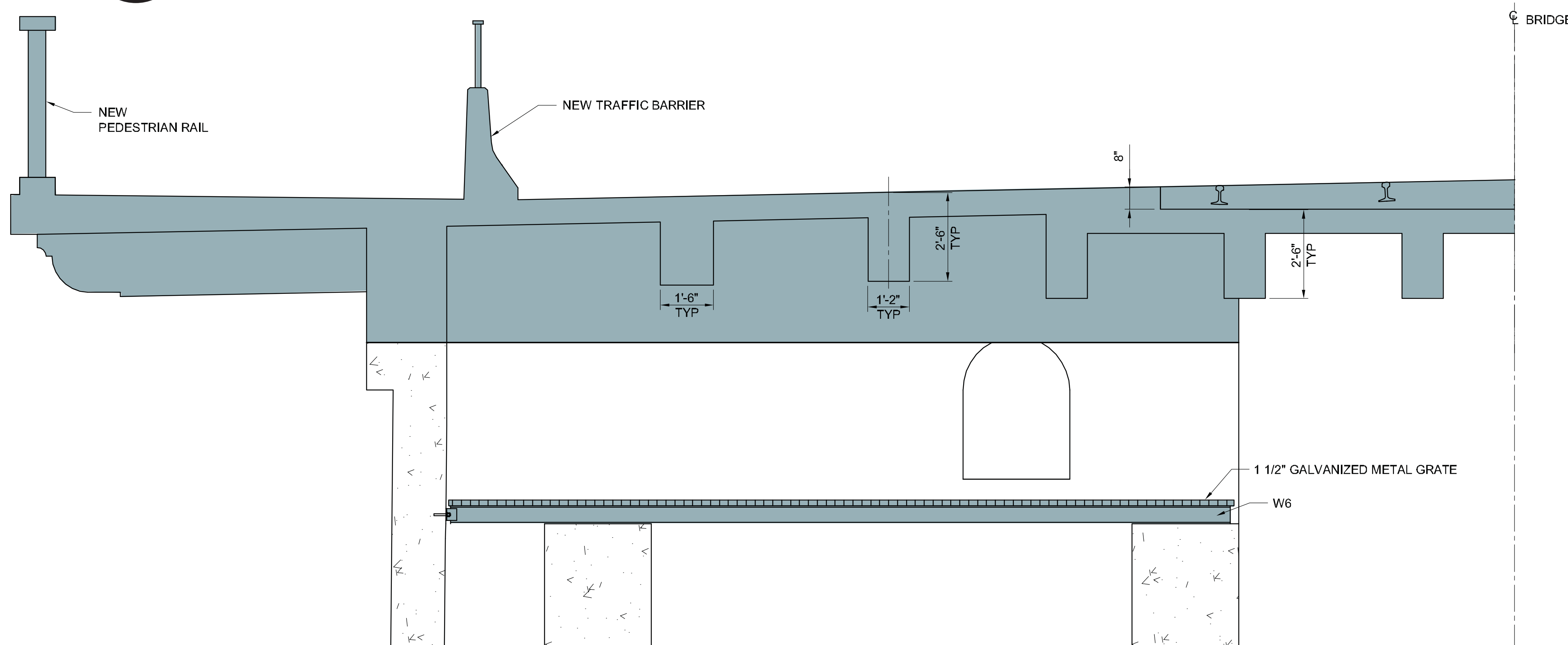
(B) Typical Pier Section (Repair)
