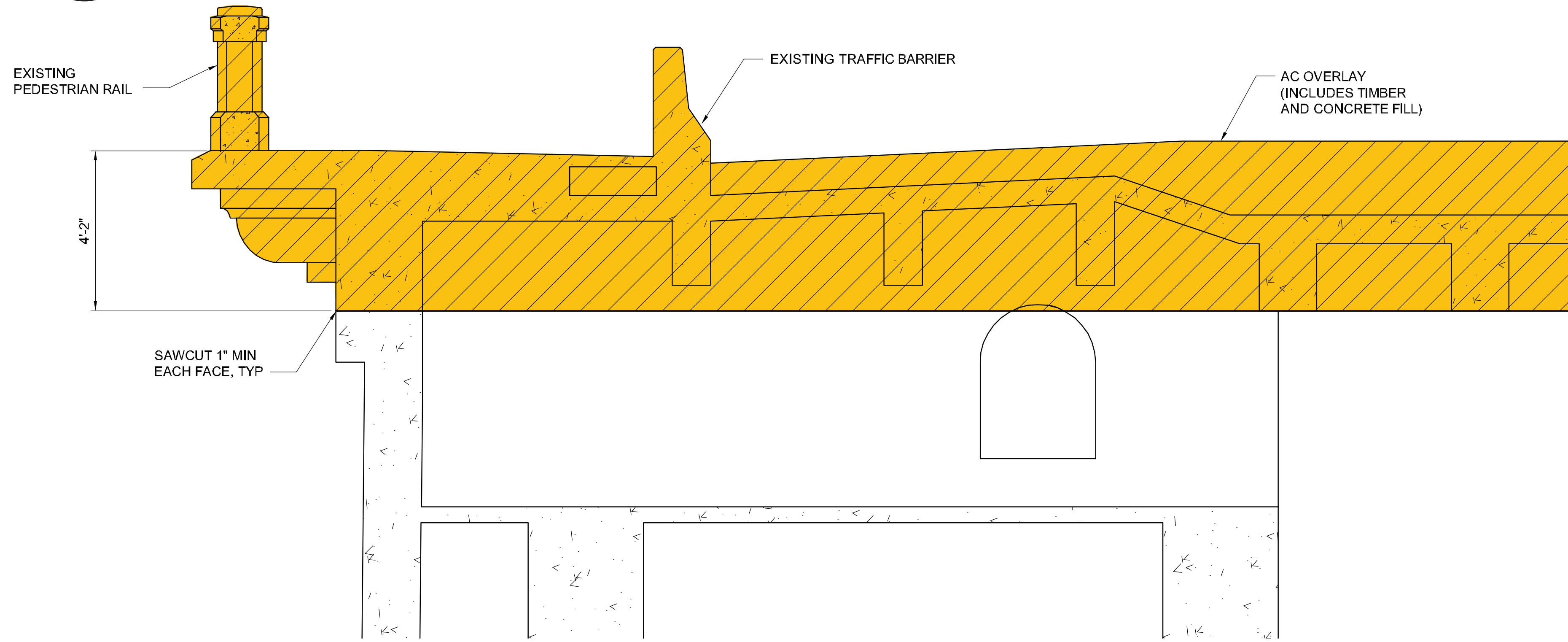
(A) Typical Deck Section (Removal)
