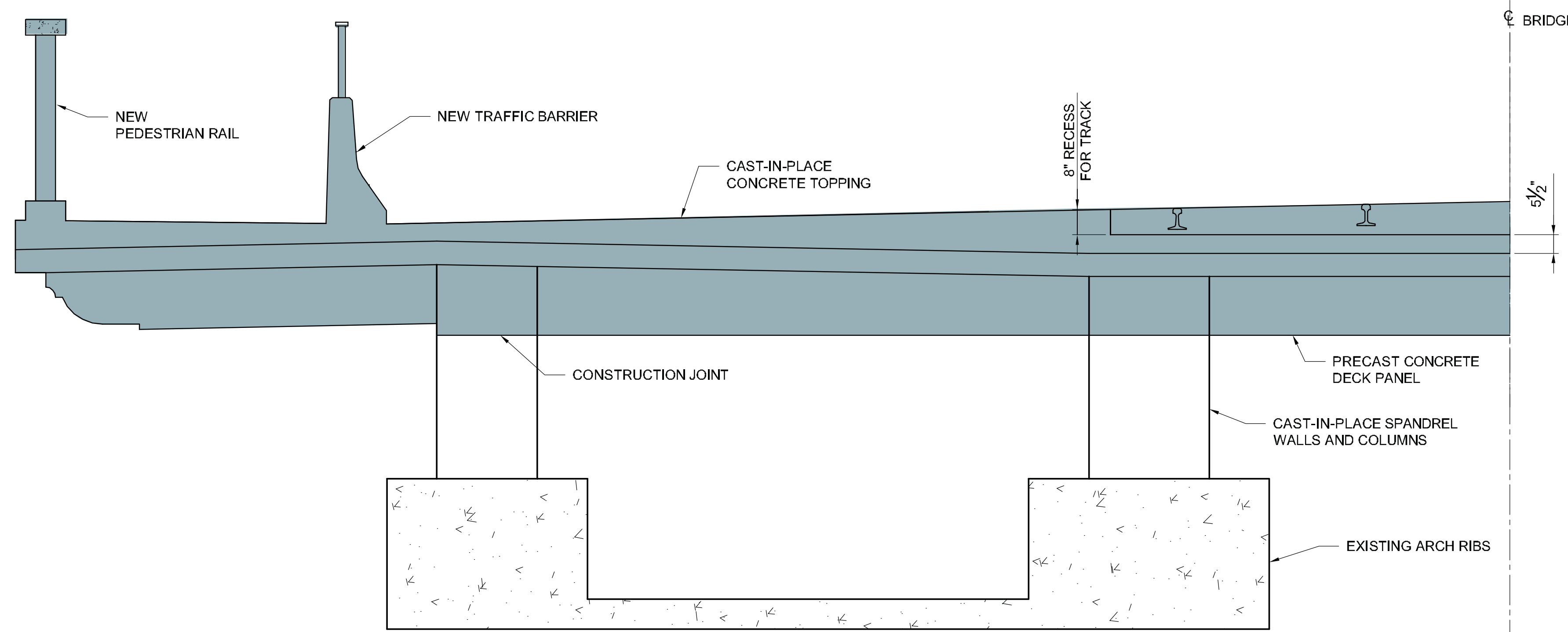
(A) Typical Deck Section (Repair)
