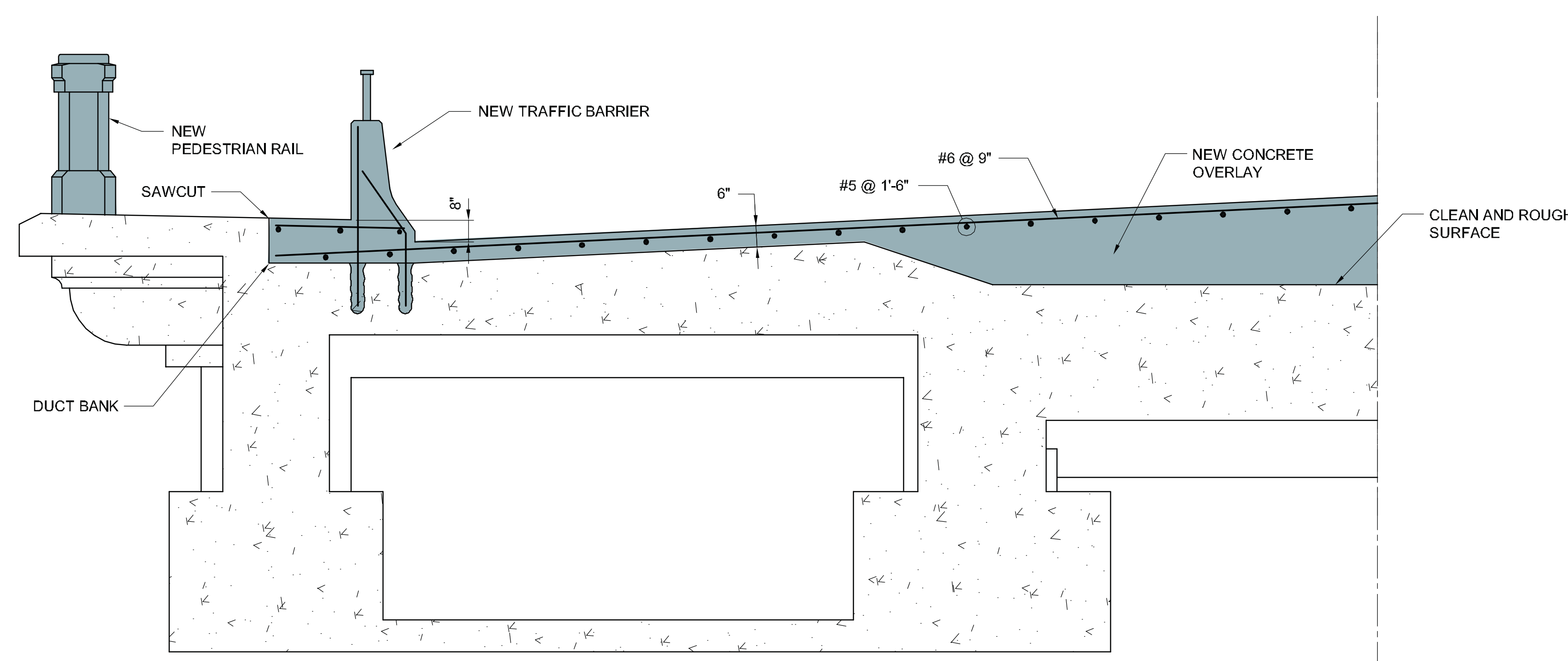
(A) Typical Deck Section (Repair)
