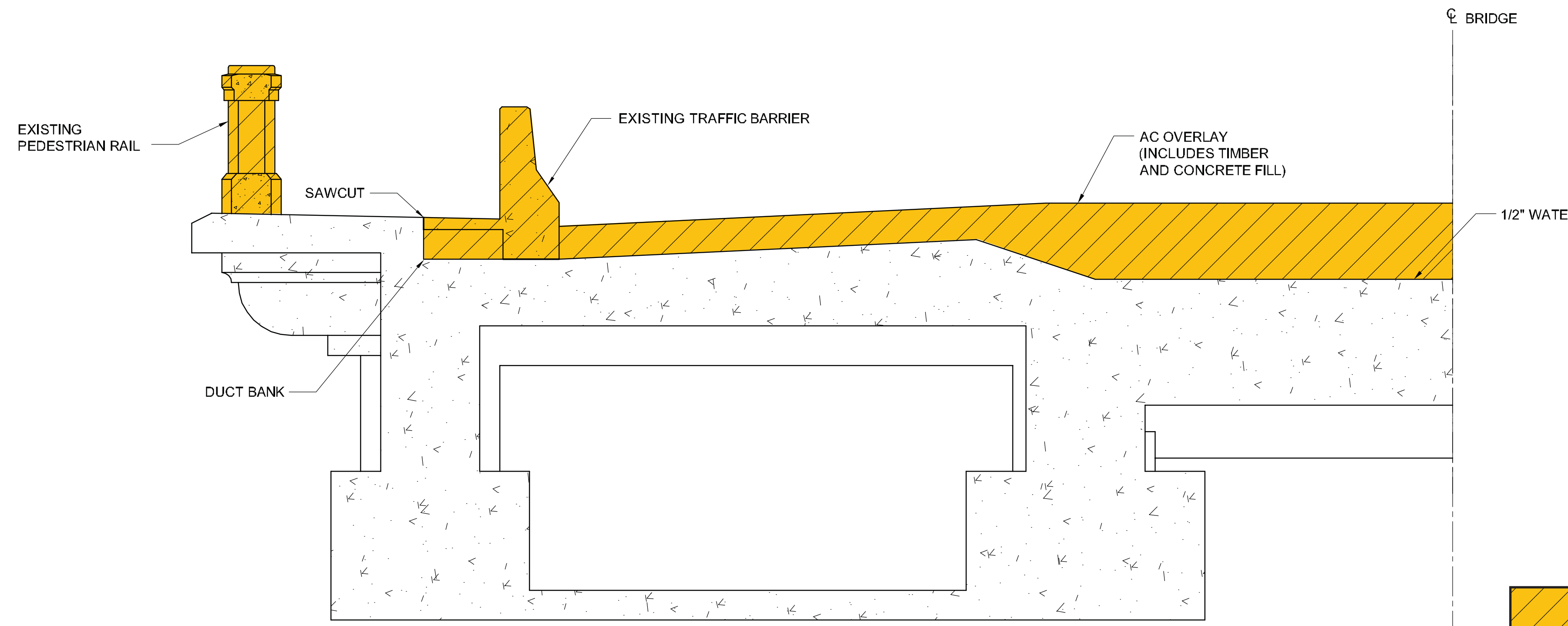
(A) Typical Deck Section (Removal)
