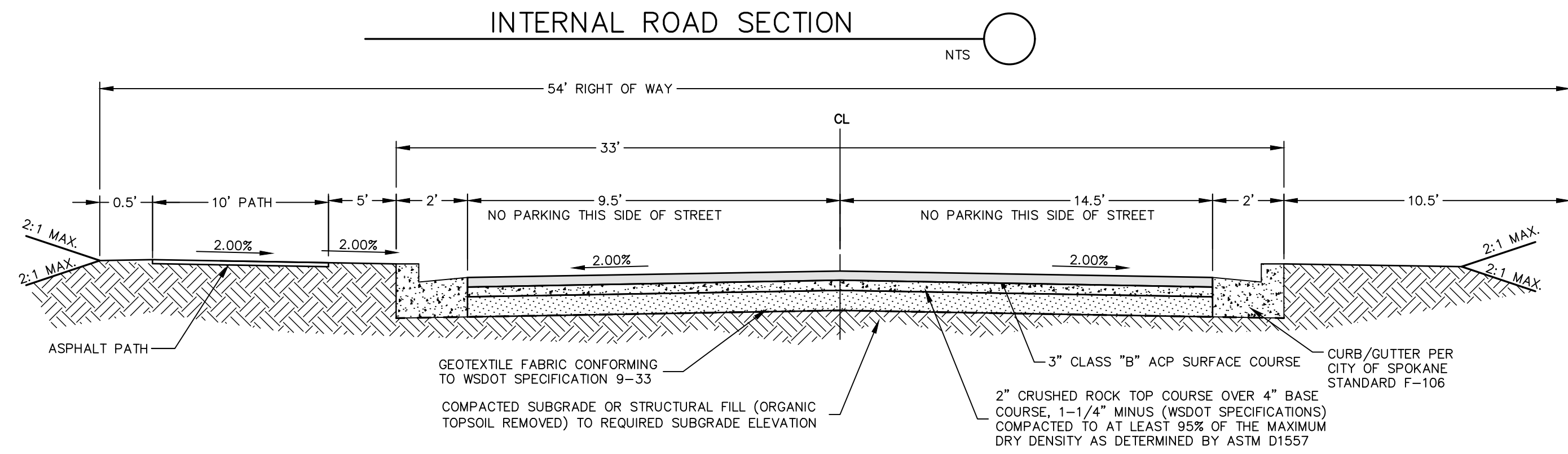
INTERNAL ROAD SECTION (SIDEWALK ON LEFT SIDE) NTS SARATOGA AVE: 30+25 TO 39+25
