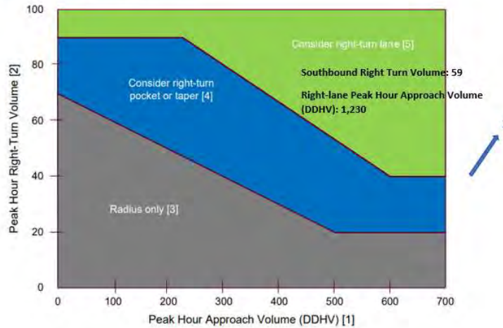
Exhibit 1310-11 Right-Turn Lane Guidelines
