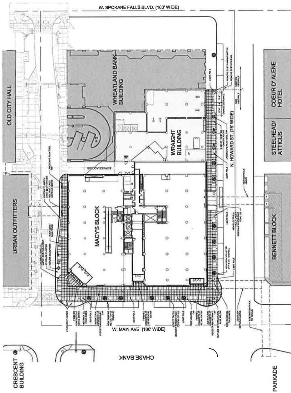
PLAN NORTH SITE PLAN Scale: 1" = 20'-0" NORTH
