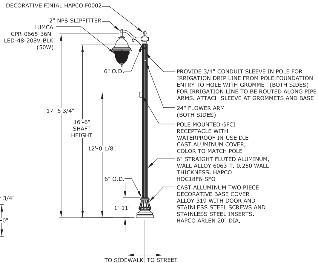
TYPE P1B
