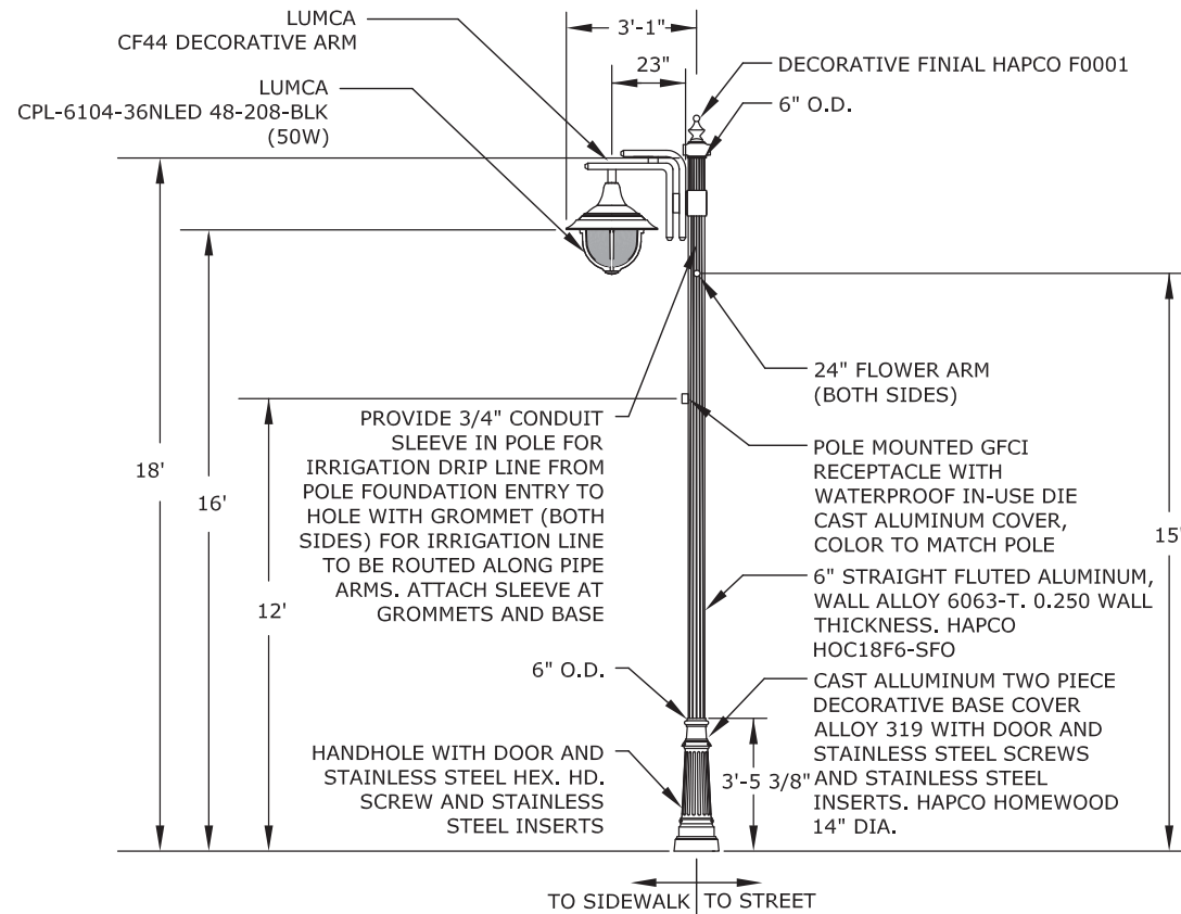
TYPE P1C
