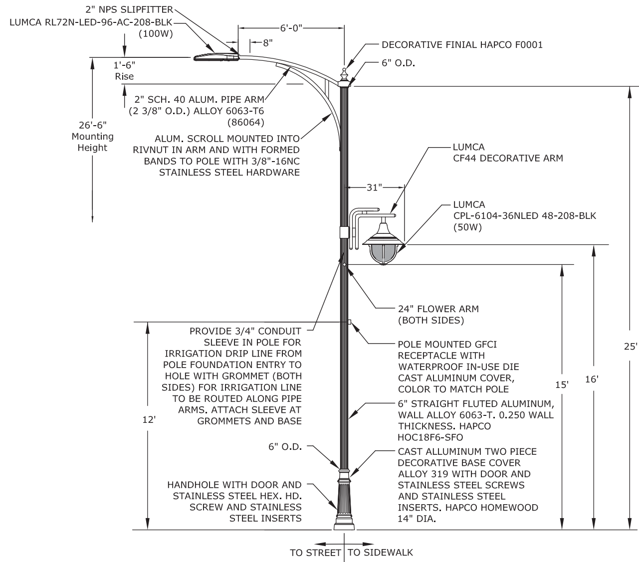
TYPE S1C
