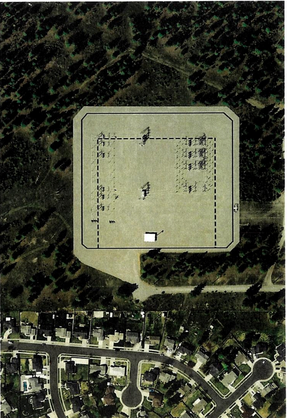
Figure 4: Expanded Substation Footprint Original footprint shown in dashed line
