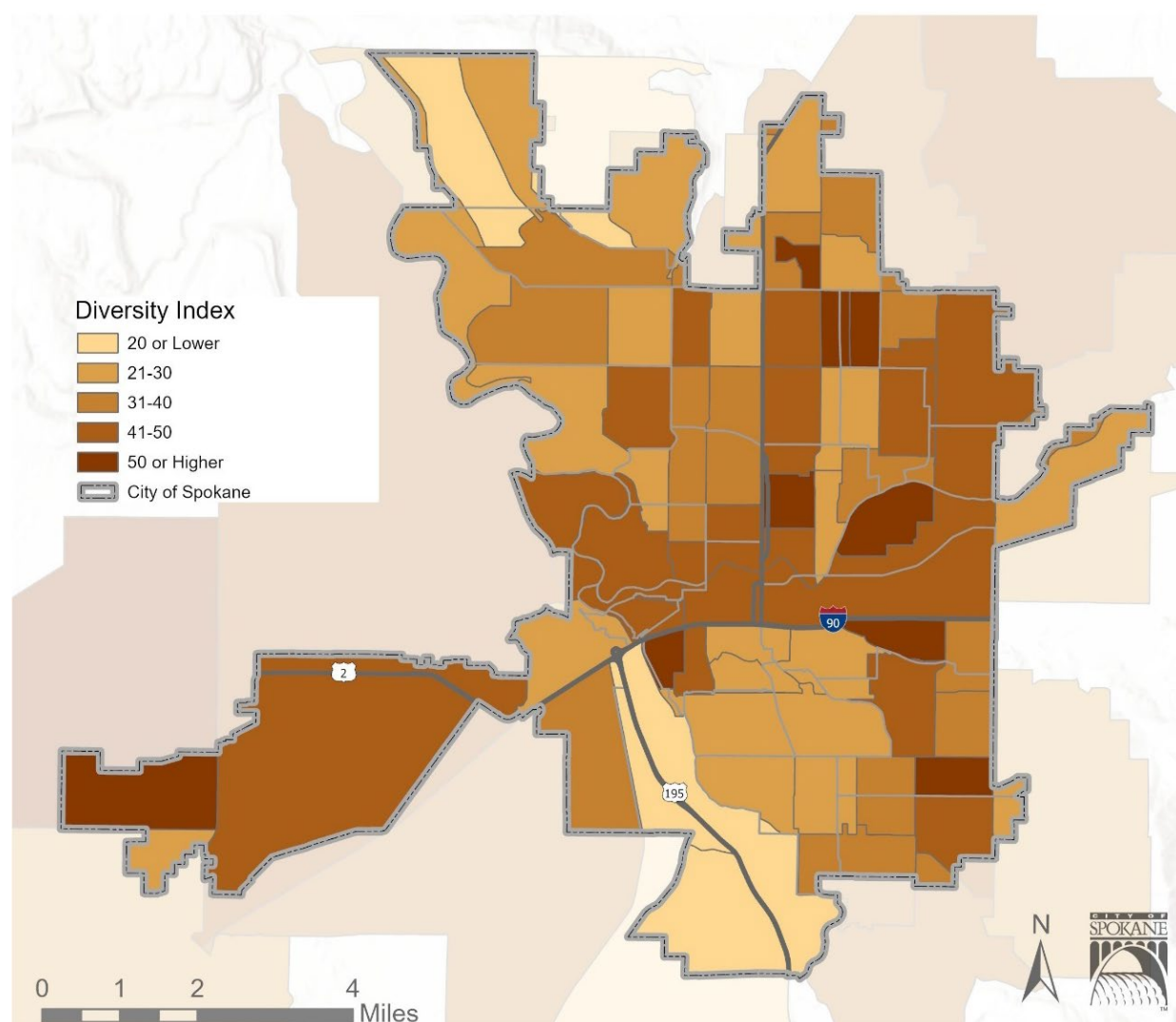
Figure 15. Diversity Index
