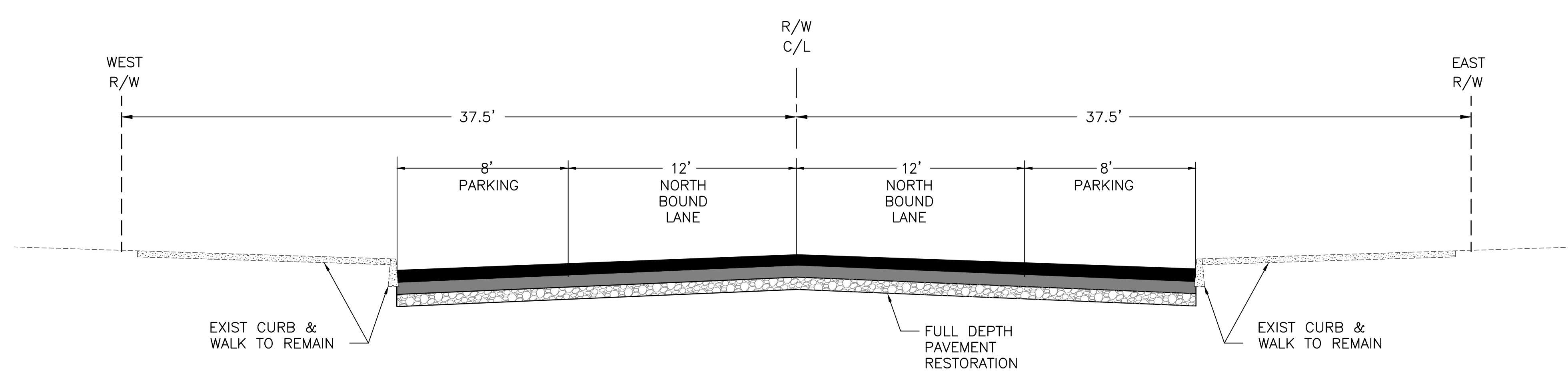
Lincoln St Section - 5th to 4th NTS
