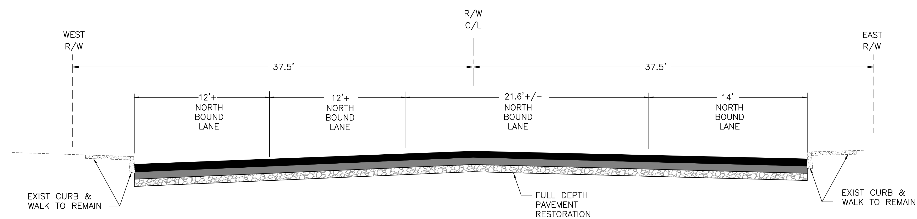
Lincoln St Section - 3rd to 4th NTS
