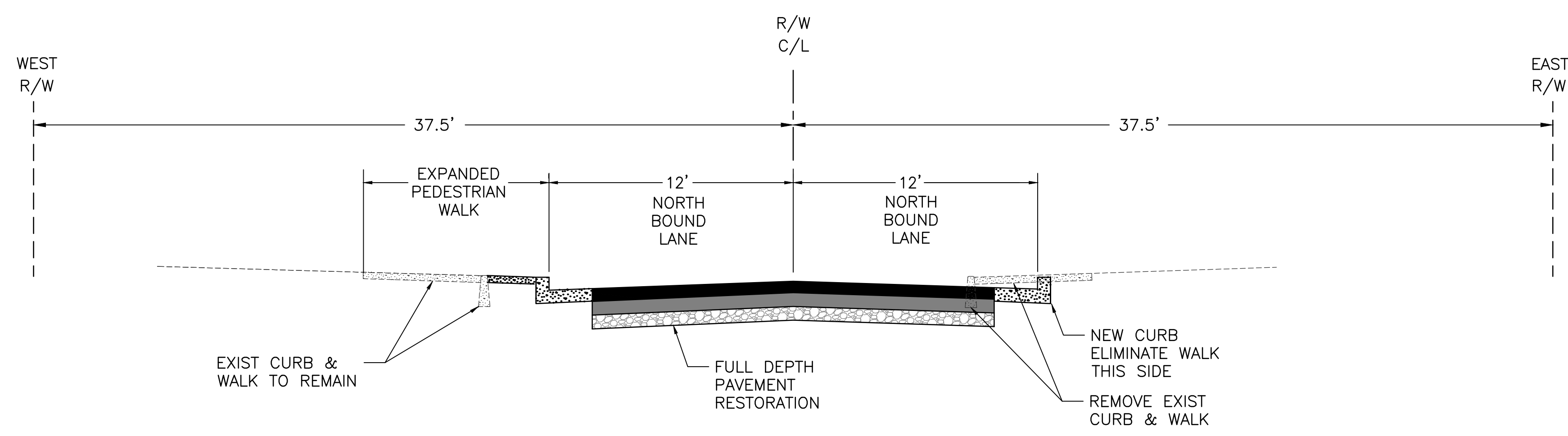
Lincoln St Section - 7th to 6th NTS
