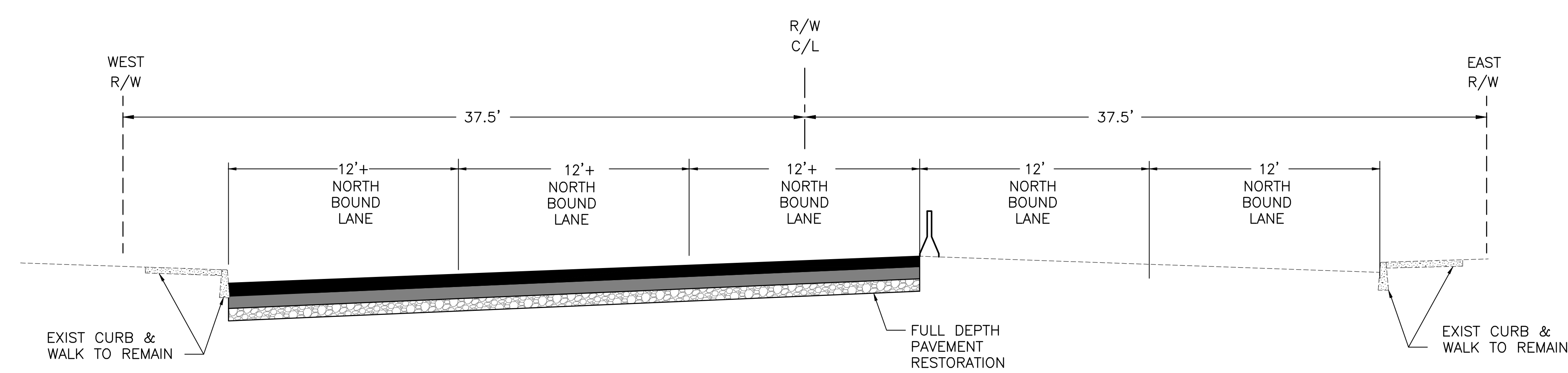
Lincoln St Section - 4th to 3rd NTS
