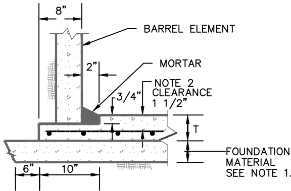
PRECAST BASE SLAB
