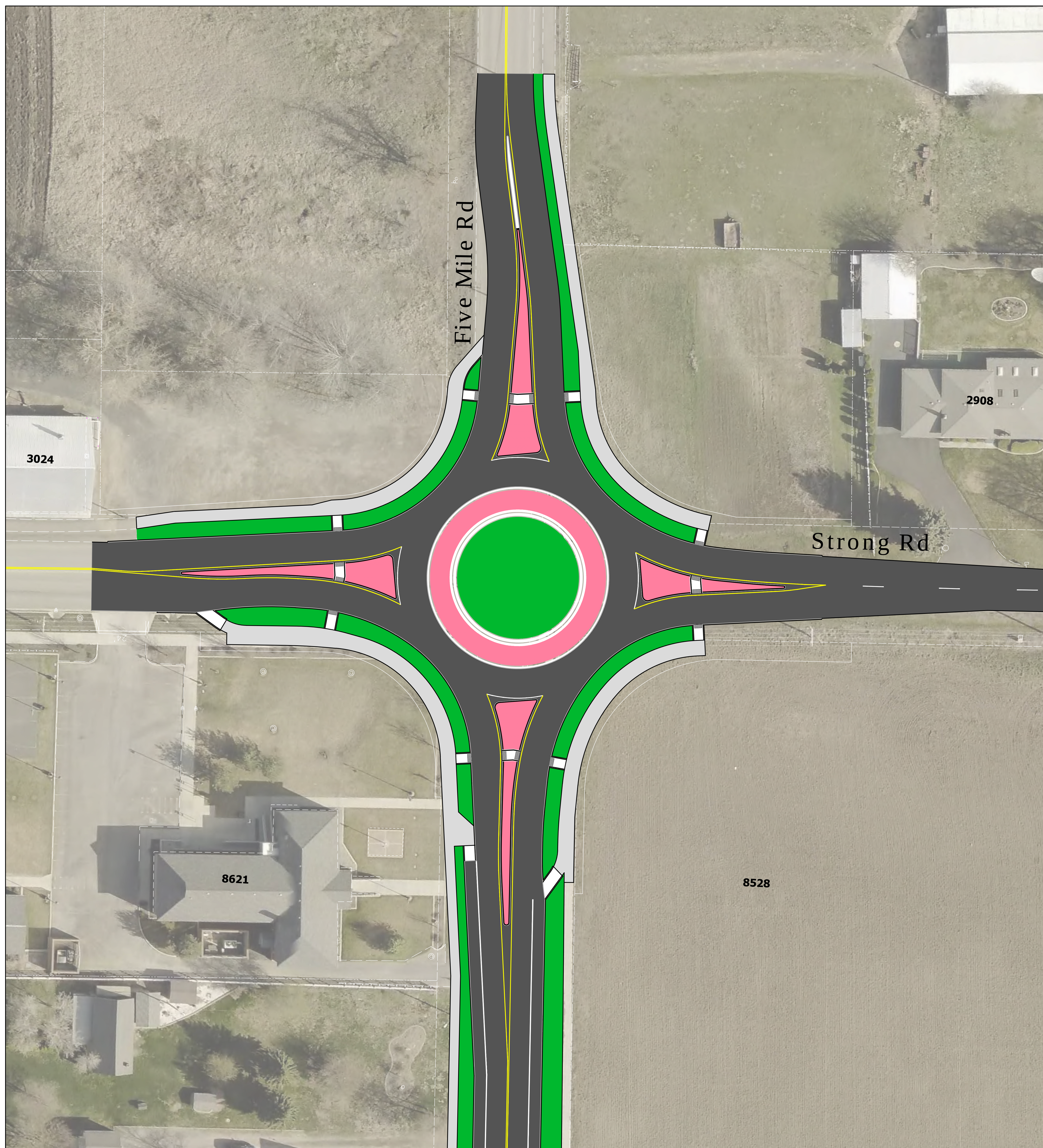
ROUNDBOUT PLAN
