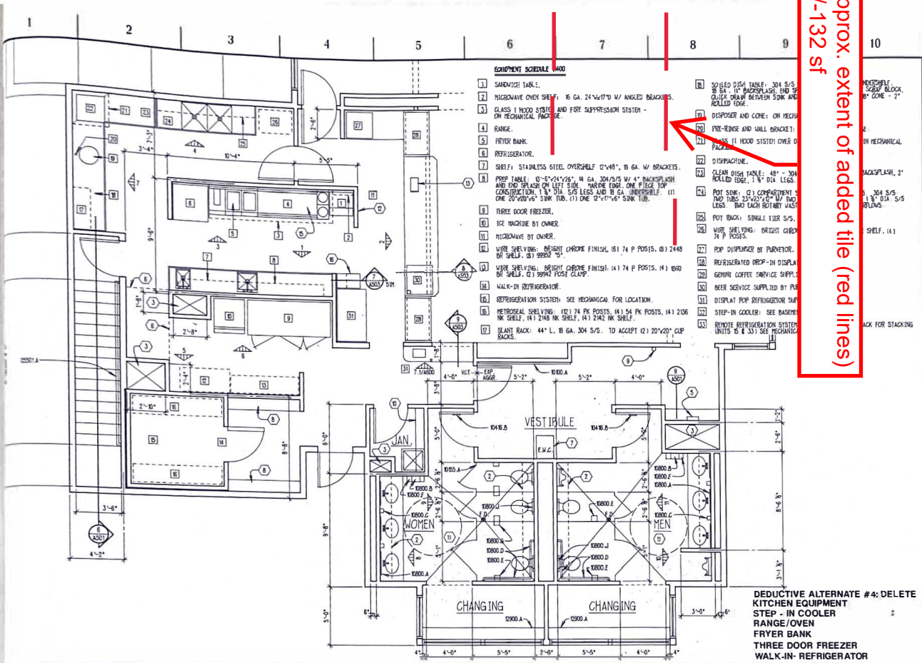
E-1 ENLARGED PLAN - KITCHEN & RESTROOM AREA
